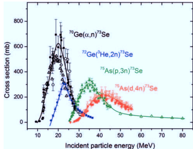
Figure 3: Excitation functions for the reactions ^{75}\text{As}(\text{p}, 3\text{n})^{73}\text{Se} , ^{75}\text{As}(\text{d}, 4\text{n})^{73}\text{Se} , ^{72}\text{Ge}(^3\text{He}, 2\text{n})^{73}\text{Se} and ^{70}\text{Ge}(\alpha, \text{n})^{73}\text{Se} drawn using the data in References [48–53].
