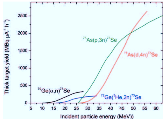
Figure 4: Thick target yields of ^{73}\text{Se} calculated from the excitation functions of ^{75}\text{As}(\text{p}, 3\text{n})^{73}\text{Se} , ^{75}\text{As}(\text{d}, 4\text{n})^{73}\text{Se} , ^{72}\text{Ge}(^3\text{He}, 2\text{n})^{73}\text{Se} and ^{70}\text{Ge}(\alpha, \text{n})^{73}\text{Se} reactions shown in Figure 3.
